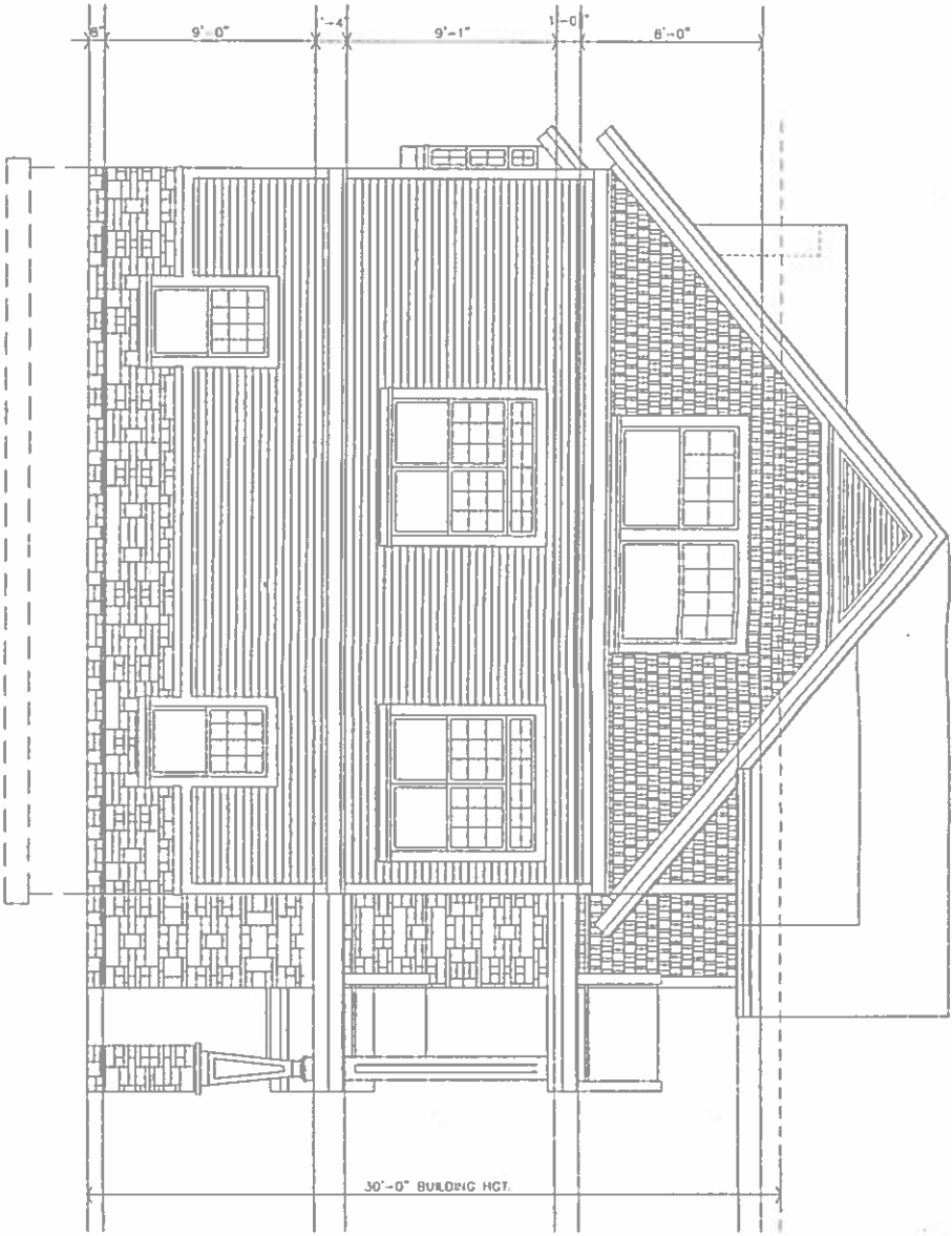
Typical Building Side Elevation
